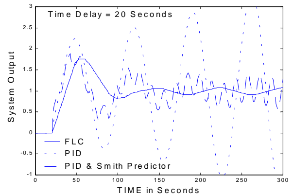
Figure 6: PID, SPC, and FLC Comparison
