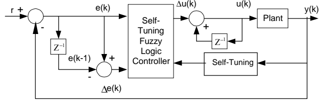
a) Closed-Loop FLC System
