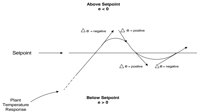
Figure 11 The Polarity of the Temperature Vector
