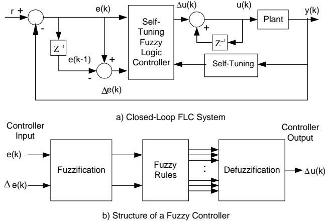
Figure 3: Fuzzy Logic Control System.
