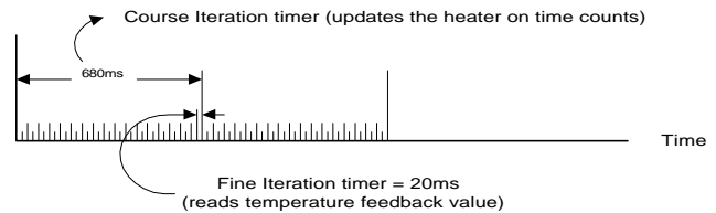
Figure 10: Local Processor Timing
