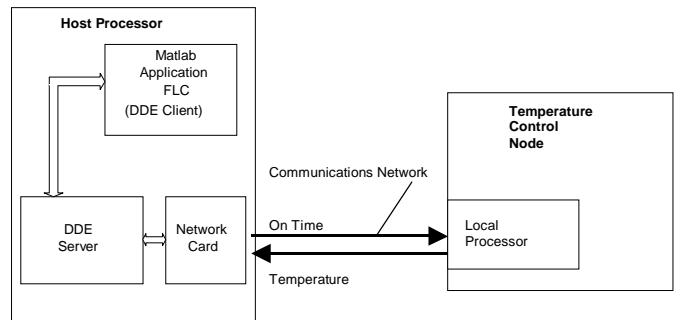
Figure 9: Distributed Control System Configuration
