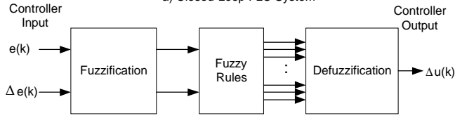
b) Structure of a Fuzzy Controller
