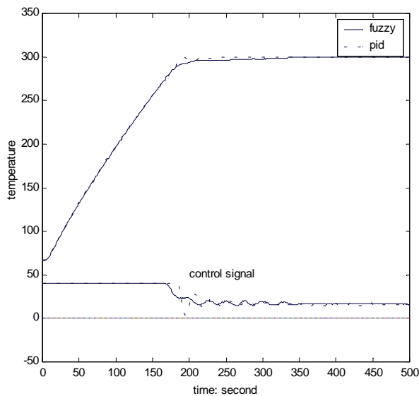
Figure 13: PID and Fuzzy Comparison at Low Temperature
