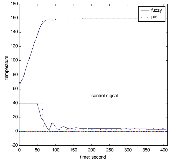
Figure 14: PID and Fuzzy Comparison with Time Delay
