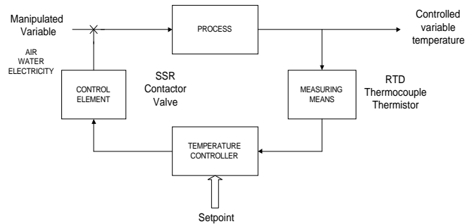
Figure 1: A typical industrial temperature control problem
