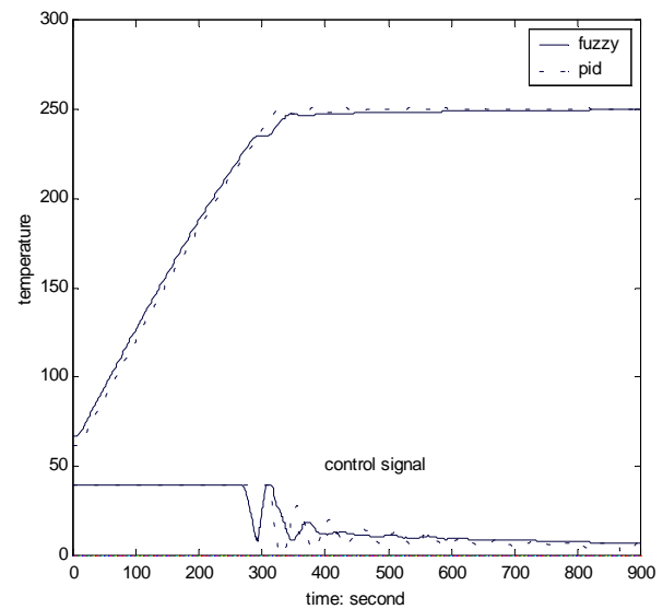
Figure 15: PID and Fuzzy Comparison with Large Thermo Mass
