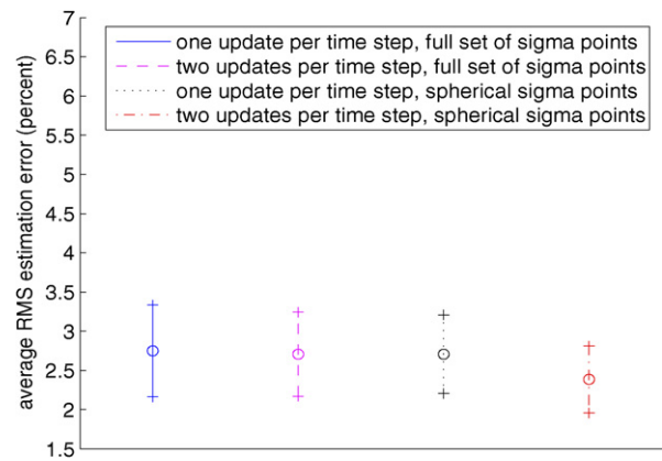
Fig. 4. Unscented Kalman filter estimation errors and standard deviations.
