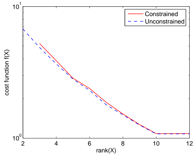
Figure 4: Constrained and unconstrained majorization results for a 12 \times 12 matrix. Constrained majorization requires \text{rank}(X) \geq 3 because of the arrangement of the constraints.
