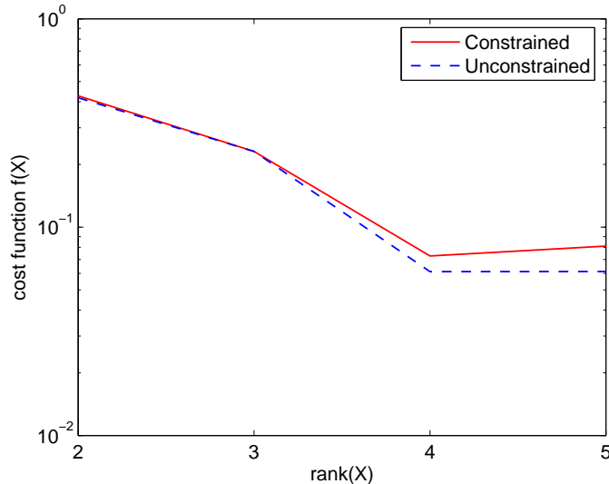
Figure 2: Constrained and unconstrained majorization results for a 5 \times 5 matrix.
