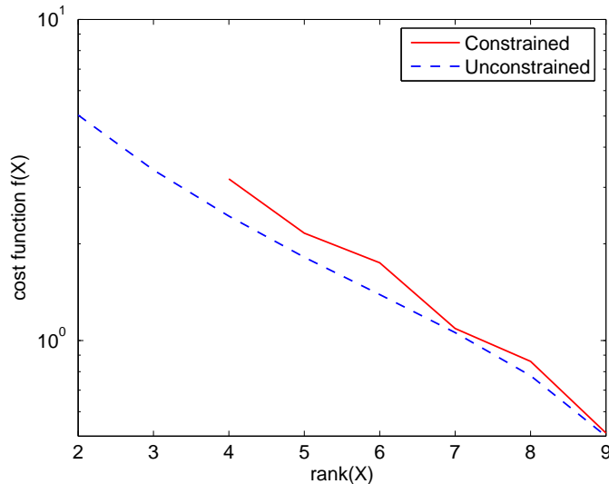
Figure 3: Constrained and unconstrained majorization results for a 10 \times 10 matrix. Constrained majorization requires \text{rank}(X) \geq 4 because of the arrangement of the constraints. Both cost functions for \text{rank}(X)=10 are zero (since R is a valid full rank correlation matrix) and so are not shown in the figure.
