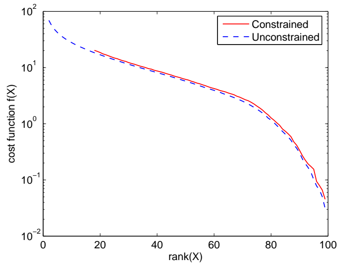
Figure 5: Constrained and unconstrained majorization results for a 100 \times 100 matrix. Constrained majorization requires \text{rank}(X) \geq 18 because of the arrangement of the constraints. Both cost functions for \text{rank}(X)=100 are zero (since R is a valid full rank correlation matrix) and so are not shown in the figure.
