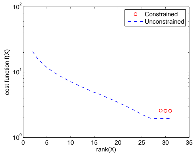
Figure 6: Constrained and unconstrained majorization results for a 31 \times 31 matrix. Constrained majorization requires \text{rank}(X) \geq 29 because of the constraints.
