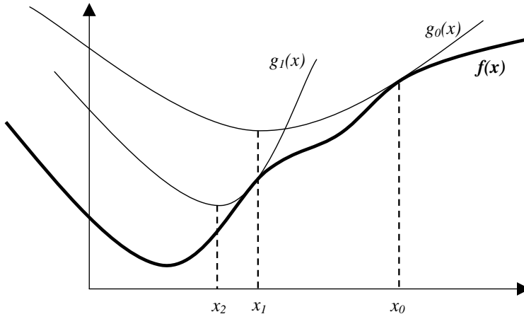
Figure 1: Illustration of majorization, adapted from [26]. The minimization process starts with an initial guess x_0 . g_0(x) is a function that matches f(x) at x = x_0 . We minimize g_0(x) to obtain x_1 . g_1(x) is a function that matches f(x) at x = x_1 . We minimize g_1(x) to obtain x_2 . The process continues until convergence.
