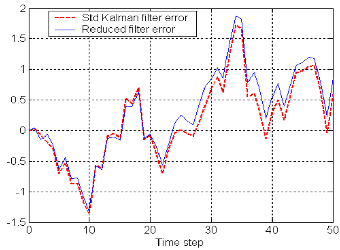
Figure 2: Error of estimate of first state element
