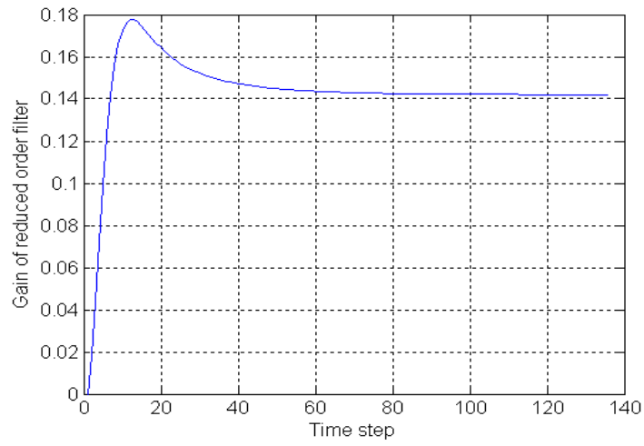
Figure 1: Convergence of reduced order gain
