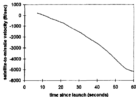
Fig. 3. Satellite-to-missile range rate.
