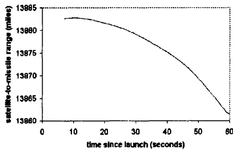
Fig. 2. Satellite-to-missile range.
