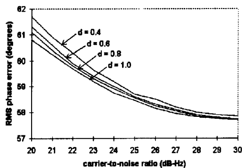
Fig. 9. RMS phase error when the PLL maintains lock. The Kalman gain was designed for CNR = 30 dB-Hz. Note that the filter is unstable for d < 0.3 .
