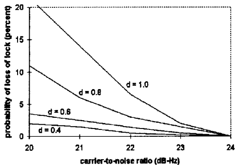
Fig. 12. Probability of loss of lock. The Kalman gain was designed for \text{CNR} = 20 dB-Hz. Note that the filter is unstable for d < 0.3 .
