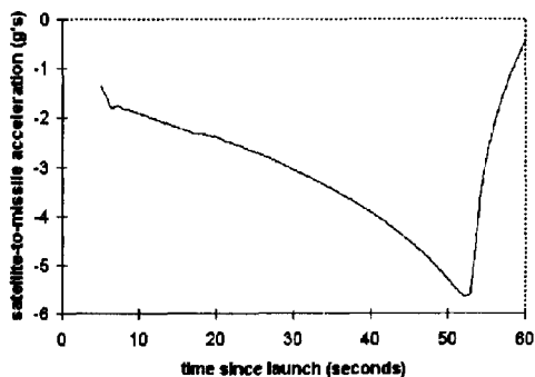
Fig. 4. Satellite-to-missile range acceleration.
