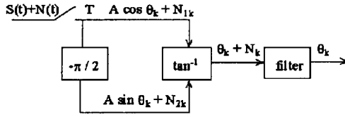
Fig. 1. Phase-locked loop architecture.
