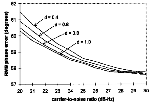
Fig. 13. RMS phase error when the PLL maintains lock. The Kalman gain was designed for \text{CNR} = 20 dB-Hz. Note that the filter is unstable for d < 0.3 .
