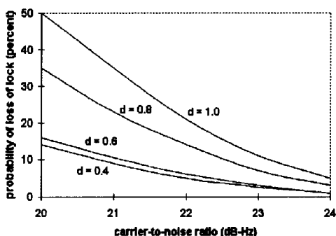
Fig. 8. Probability of loss of lock. The Kalman gain was designed for CNR = 30 dB-Hz. Note that the filter is unstable for d < 0.3 .
