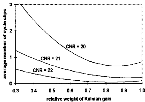
Fig. 11. Average number of cycle slips when the PLL maintains lock. The Kalman gain was designed for \text{CNR} = 20 dB-Hz. Note that the filter is unstable for d < 0.3 .
