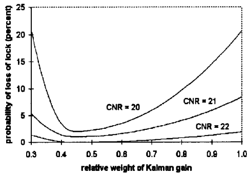
Fig. 10. Probability of loss of lock. The Kalman gain was designed for \text{CNR} = 20 dB-Hz. Note that the filter is unstable for d < 0.3 .
