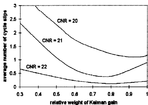
Fig. 7. Average number of cycle slips when the PLL maintains lock. The Kalman gain was designed for CNR = 30 dB-Hz. Note that the filter is unstable for d < 0.3 .
