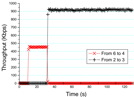
Fig 4. Throughput of two TCP connections with different sender and receiver, window\_ = 4
