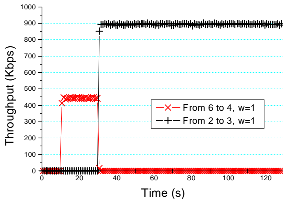
Fig 5. Throughput of two TCP connections with different sender and receiver, window\_ = 1
