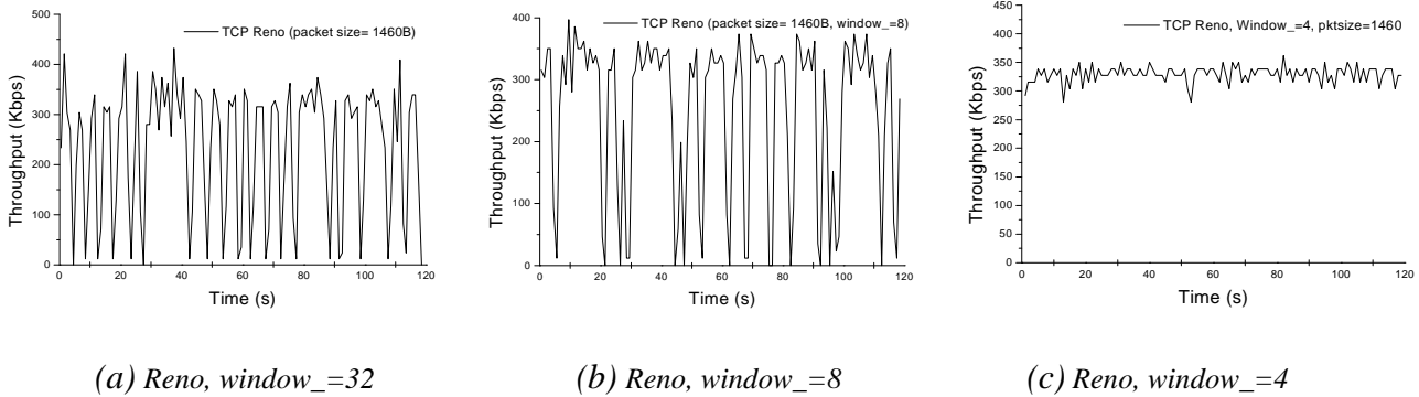
Figure 2. Instability problem in the four hops TCP connection. (from node 1 to node 5.) TCP packet size = 1460B
