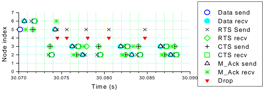
Fig 8. Part of the MAC layer packet trace in the “W1 run”. window_=1
