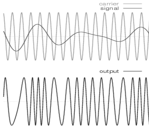
Figure 1-FM modulation.
