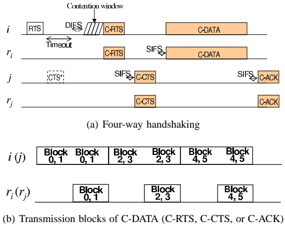
Fig. 3. A simple cooperation scheme with partners r_i and r_j on a weak link ( i, j ). (SIFS or short interframe space and DIFS or DCF interframe space are the spaces between frames in the four-way handshaking procedure. The DATA frame in this figure consists of 6 blocks.)
