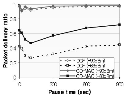
(a) Packet delivery ratio
