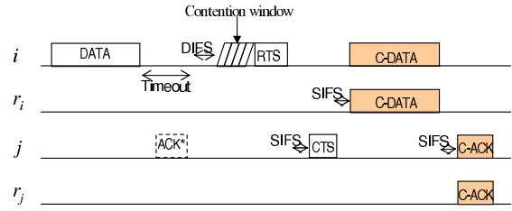
(a) Four-way handshaking
