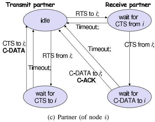
Fig. 5. State transition diagrams for a sender, a receiver and a partner. (Figure (c) shows the state transitions of a transmit partner as well as a receive partner.)
