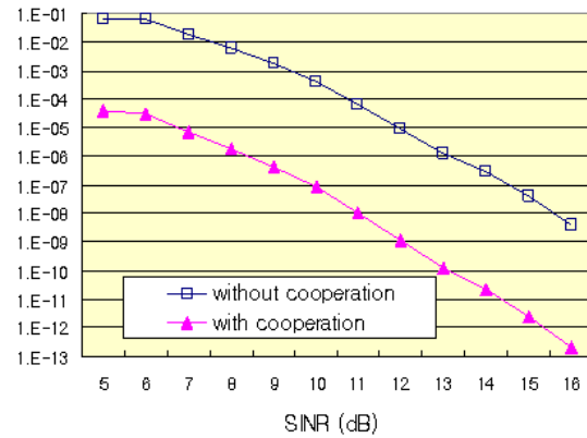
(a) BER versus SINR
