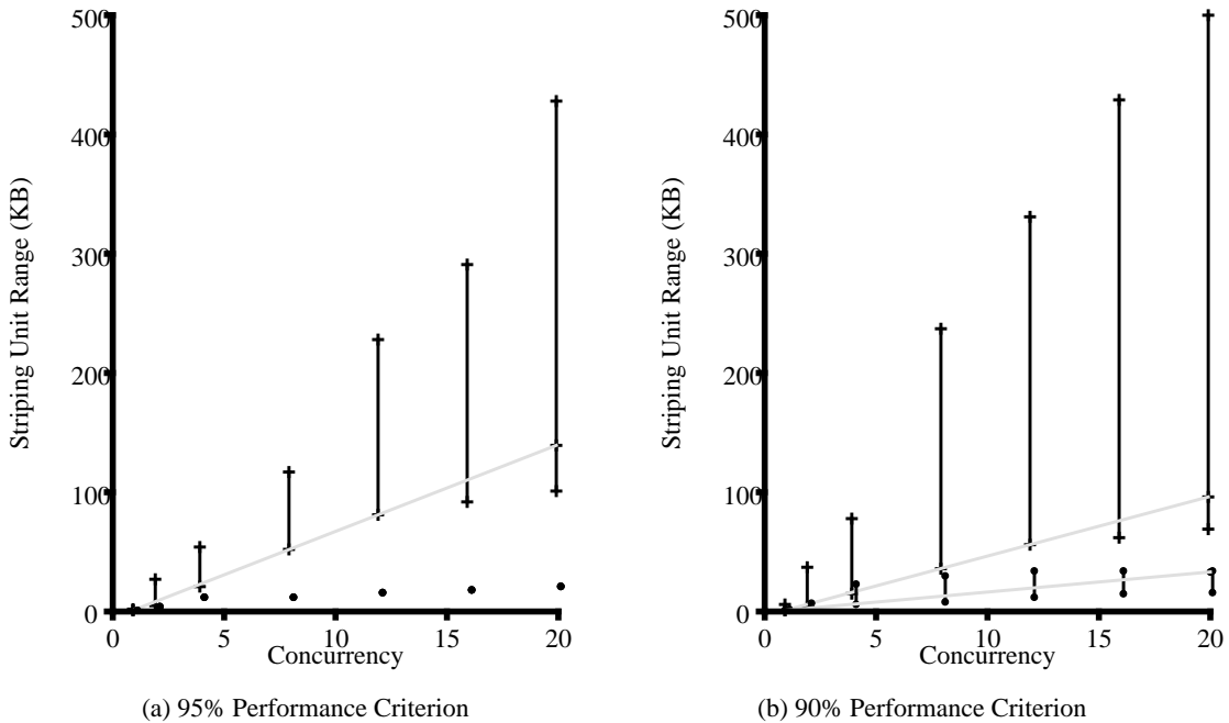
Figure 6: Striping Unit Chosen Versus Concurrency—17 IBM Lightning Disks. Shown here is the range of striping units which yield at least 95% (Figure a) or 90% (Figure b) of the maximum throughput for all request sizes (exp4KB, exp16KB, norm100KB, norm400KB, norm1500KB) for reads and writes. The range for a workload with 100% reads is wider and marked by + signs. The range for workloads with 100% writes is much narrower and marked by • signs. Write workloads are not always able to attain 95% performance, so Figure a shows the striping unit that yields the highest performance for all workloads (which is always at least 93%). The dashed lines are the lines with smallest slope that lie entirely in the striping unit range.
