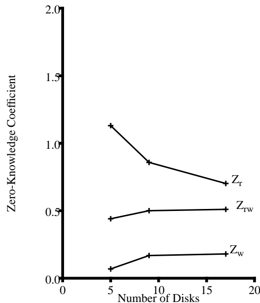
Figure 7: How Striping Units Vary with Number of Disks. This figure shows that the zero-knowledge coefficients Z_r , Z_w , and Z_{rw} vary differently with the number of disks. Since the striping unit is directly proportional to Z , the best striping unit varies in the same way as the various Z coefficients. For read-intensive workloads, Z_r decreases as the number of disks increases because smaller striping units are needed to ensure that all disks are used. For write-intensive workloads, Z_w decreases as the number of disks decreases because the extra overhead of read-modify writes becomes prohibitive when there are less disks. These two trends effectively cancel each other out, and so the overall choice of striping unit without knowing the read/write mix is approximately 0.5 and is independent of the number of disks. The optimal striping units using the values of Z_{rw} shown here guarantees approximately 60% of maximum throughput to all workloads. For read-intensive workloads, a striping unit derived from Z_r guarantees approximately 70% of maximum throughput for all workloads. For write-intensive workloads, a striping unit derived from Z_w guarantees approximately 70% of maximum throughput.
