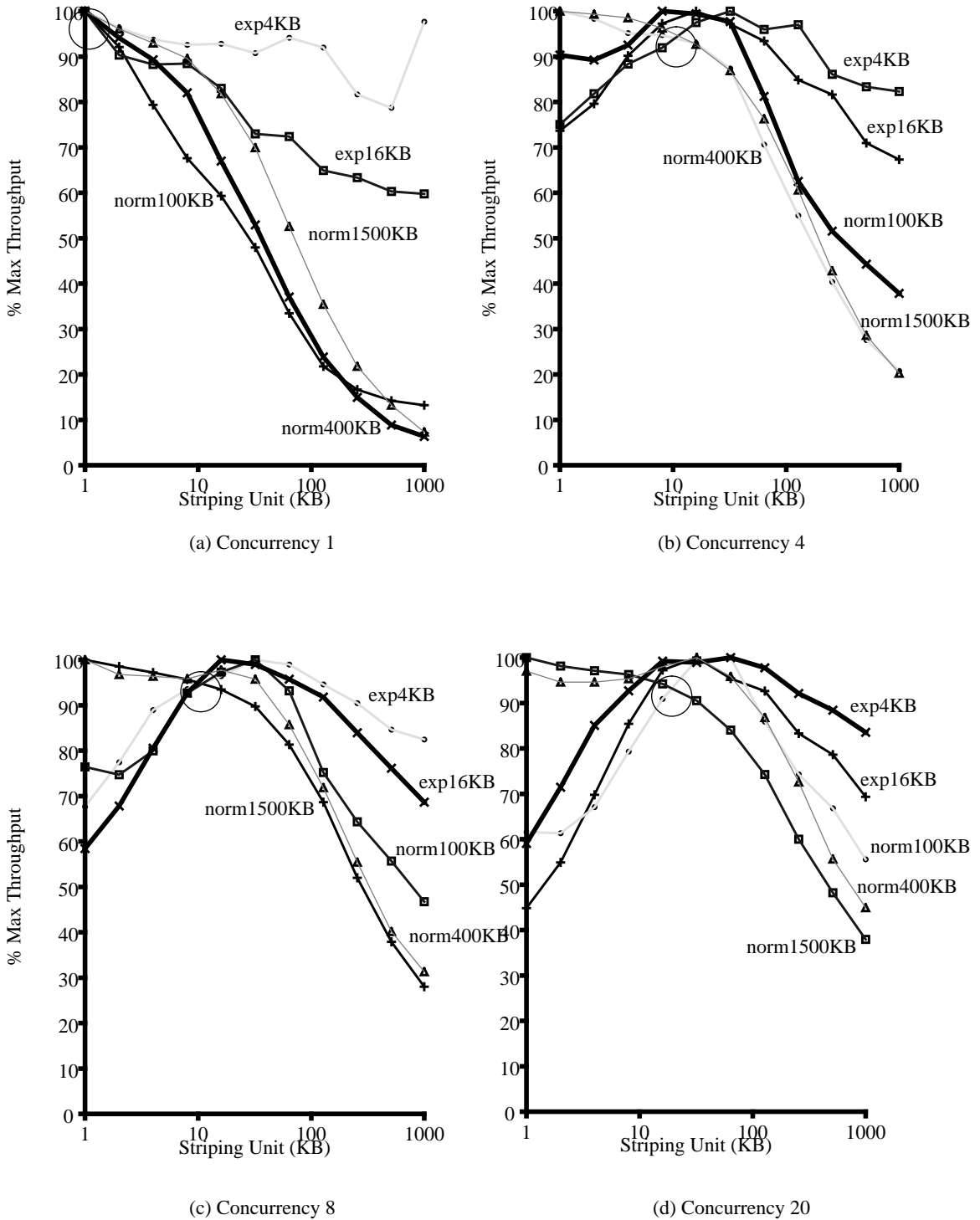
Figure 5: Write Performance for a Range of Sizes and Concurrency, Shown as Percentage of Maximum Throughput. Percentage of maximum throughput is shown as a function of the striping unit. The circled point on each graph indicates the striping unit that guarantees the highest percentage of maximum throughput to all workloads shown on that graph. Note that the optimal striping unit for write-intensive workloads is smaller than for the read-intensive workloads in Figure 4.
