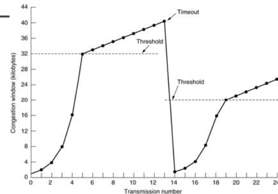
An example of the Internet congestion algorithm
